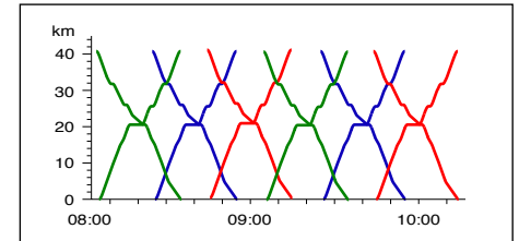
Train Graph
